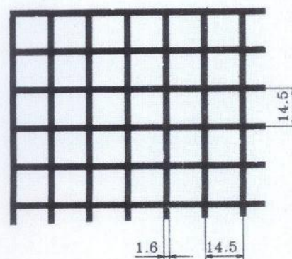
Polystyrene Egg Crate Core suffix "P" size 14.5mm x 14.5mm x 1.6mm free area = 80%
