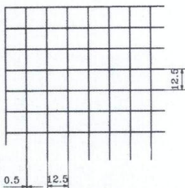
Aluminium Egg Crate Core suffix "A" size 12.5mm x 12.5mm x 0.5mm free area = 90%
